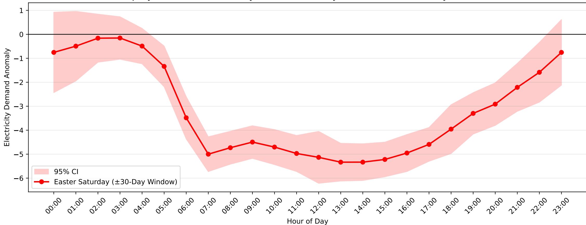
Top Ryde Demand Anomaly: Easter Saturday (2004-2017, \pm 30 -Day Window)
